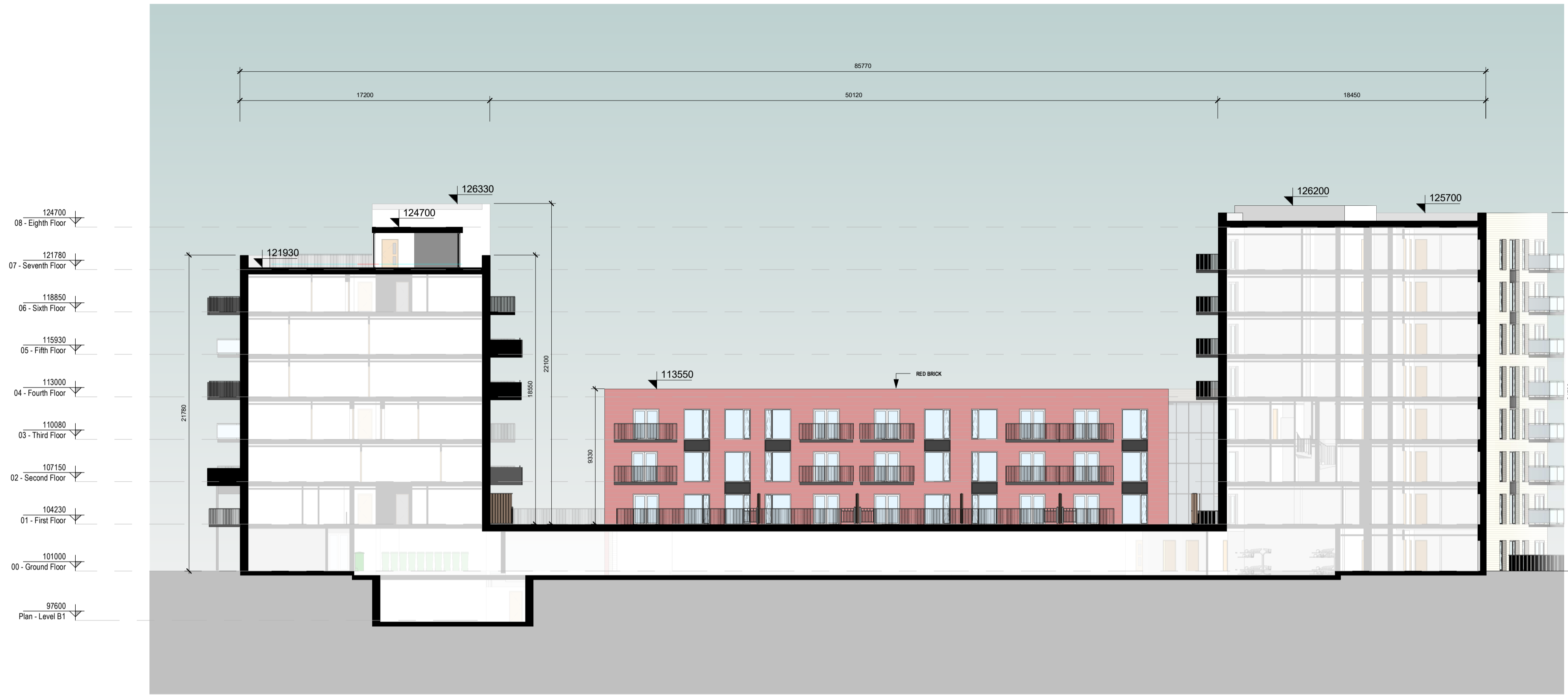
1 Block A - Elevation A7 1 : 200
